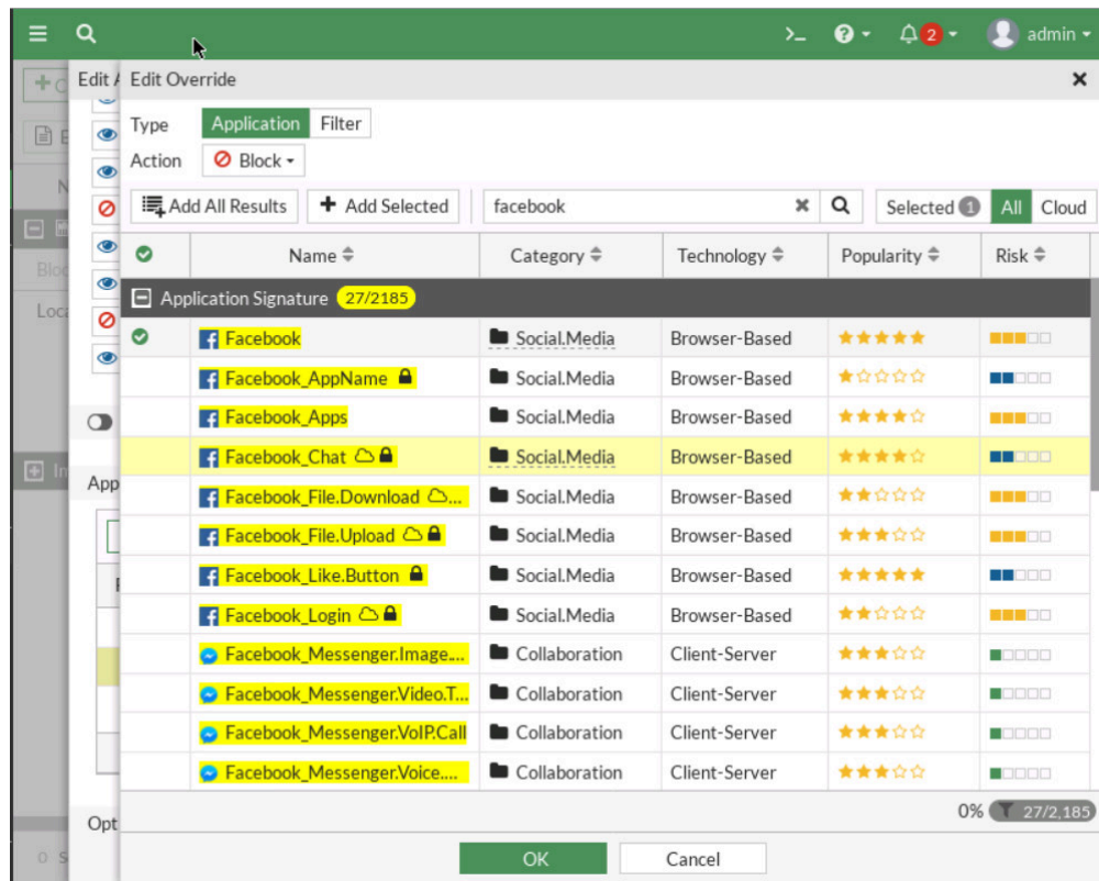
Figure 2.19: Block Facebook
