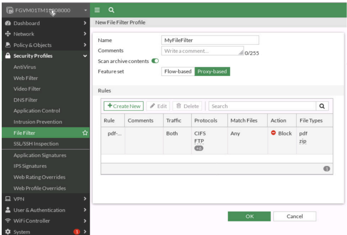
Figure 7.14: Blocking Pdf-Zip
