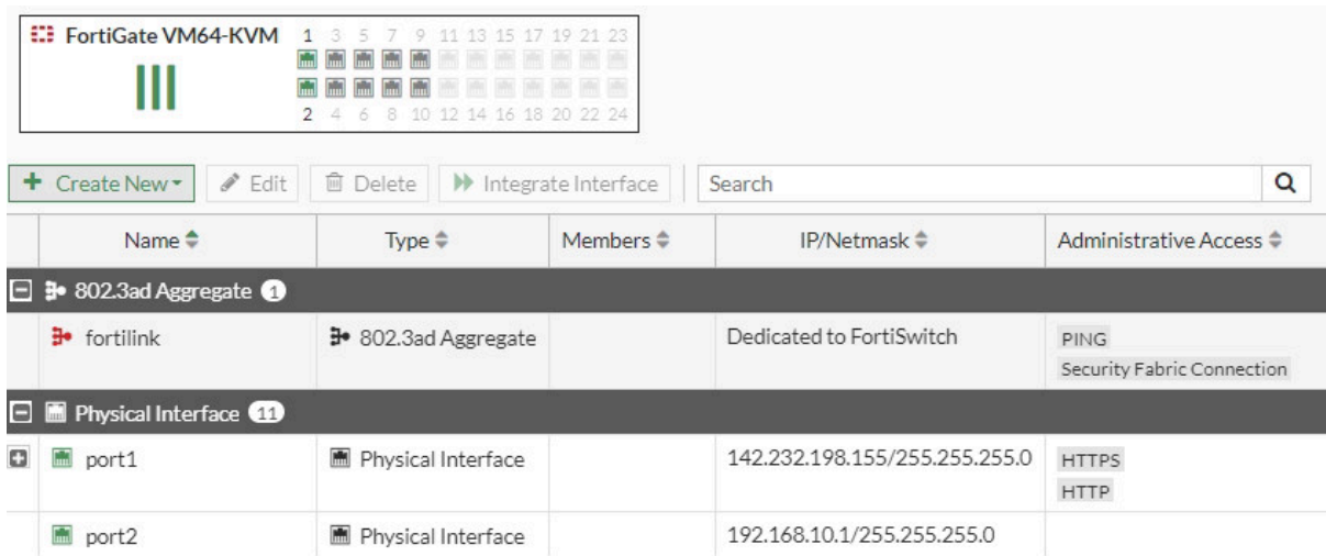
Figure 10.155: Firewall interfaces
