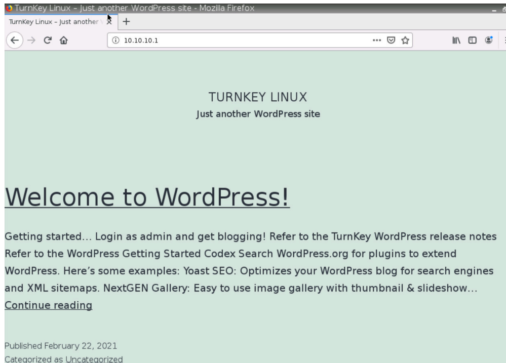
Figure 3.11: Verify configuration
