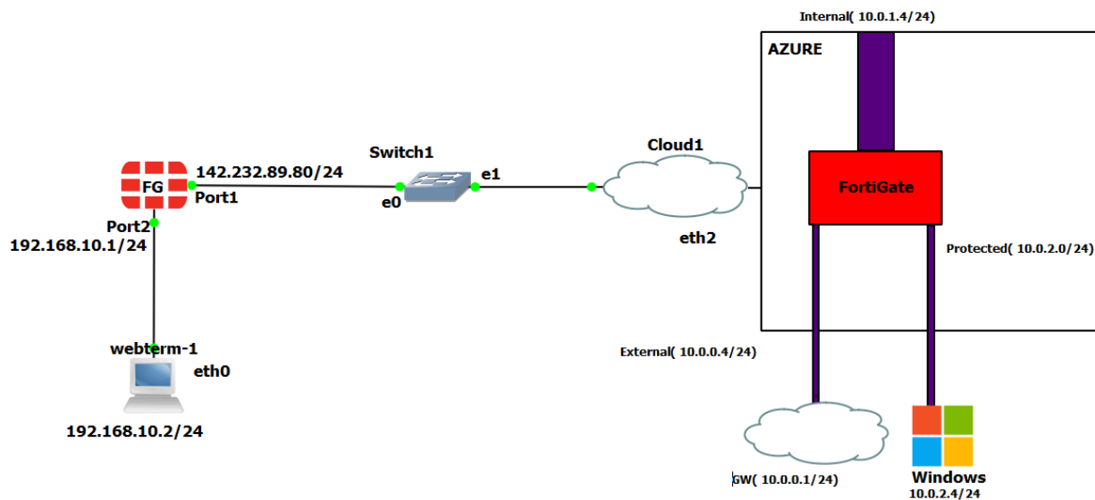
Figure 10.49: Main scenario
