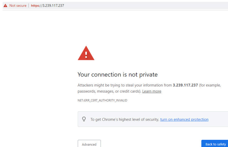
Figure 10.147: Access FortiGate
