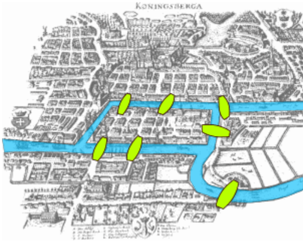
Figure 1. Map of Königsberg in Euler's time showing the actual layout of the seven bridges, highlighting the river Pregel and the bridges. Source: Königsberg bridges by Bogdan Giuşcă ( http://creativecommons.org/licenses/by-sa/3.0/deed.en ) licensed under CC BY SA 3.0 ( http://creativecommons.org/licenses/by-sa/3.0/deed.en )
