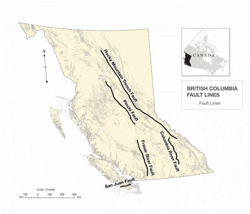
Figure 8.8 British Columbia fault lines
