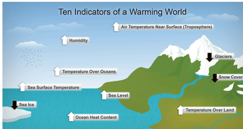
Figure 8.4 Ten indicators of a warming world
