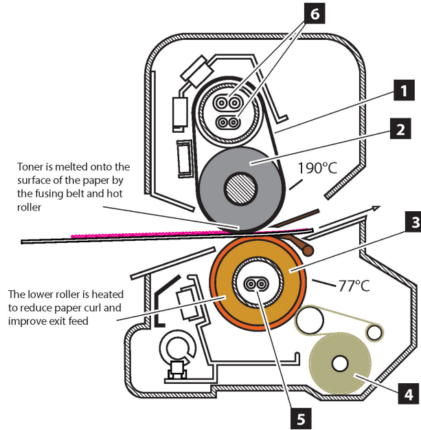
Fuser
