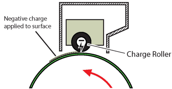
( http://opentextbc.ca/graphicdesign/wp-content/uploads/sites/42/2015/11/EP-Imaging-System-Charging.jpg ) Figure 6.5 Charge roller
