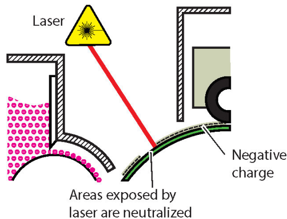
( http://opentextbc.ca/graphicdesign/wp-content/uploads/sites/42/2015/11/EP-Imaging-System-Exposure.jpg ) Figure 6.6 Exposure
