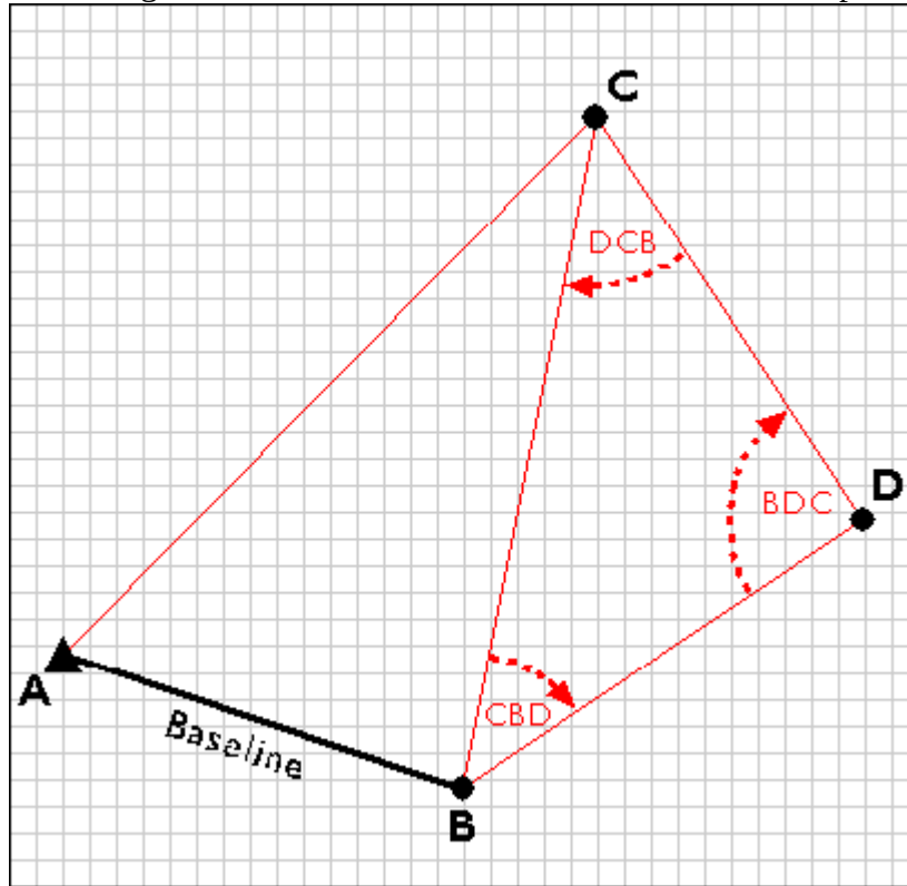
Extending the triangulation network.
