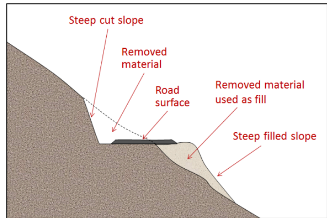
Figure 15.3.1 An example of a road constructed by cutting into a steep slope. The cut material was moved to outside part of the road to act as fill.
