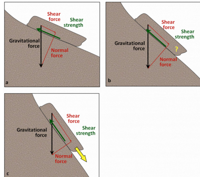
Figure 15.1.1 Differences in the shear and normal components of the gravitational force on slopes with differing steepness. The gravitational force is the same in all three cases. In (a) the shear force is substantially less than the shear strength, so the block should be stable. In (b) the shear force and shear strength are about equal, so the block may or may not move. In (c) the shear force is substantially greater than the shear strength, so the block is very likely to move.
