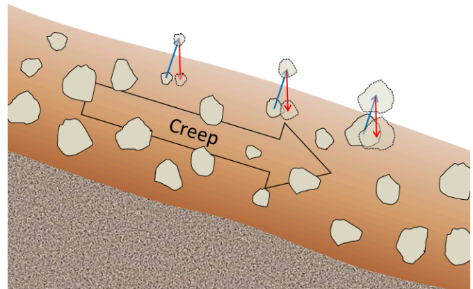
Figure 15.2.6 A depiction of the contribution of freeze-thaw to creep. The blue arrows represent uplift caused by freezing in the wet soil underneath, while the red arrows represent depression by gravity during thawing. The uplift is perpendicular to the slope, while the drop is vertical.
