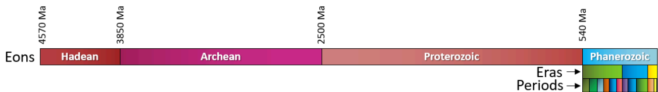
Figure 8.1.2 The four eons of Earth’s history.
