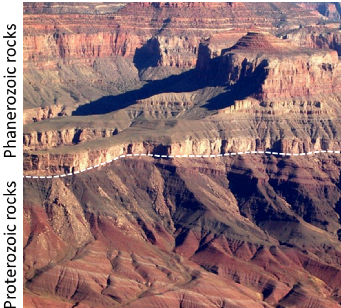
Figure 8.2.4 The great angular unconformity in the Grand Canyon, Arizona. The tilted rocks at the bottom are part of the Proterozoic Grand Canyon Group (aged 825 to 1,250 Ma). The flat-lying rocks at the top are Paleozoic (540 to 250 Ma). The boundary between the two represents a time gap of nearly 300 million years.
