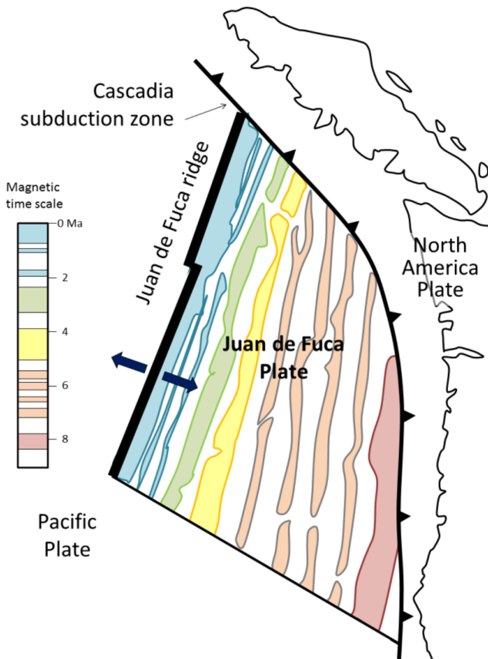
Figure 8.5.5 The pattern of magnetism within the area of the Juan de Fuca Plate, off the west coast of North America. The coloured shapes represent parts of the sea floor that have normal magnetism, and the magnetic time scale is shown using the same colours. The blue bands represent Brunhes, Jaramillo, and Olduvai; the green represents Gauss; and so on. (Note that in this diagram, sea-floor magnetism is only shown for the Juan de Fuca Plate, although similar patterns exist on the Pacific Plate.)
