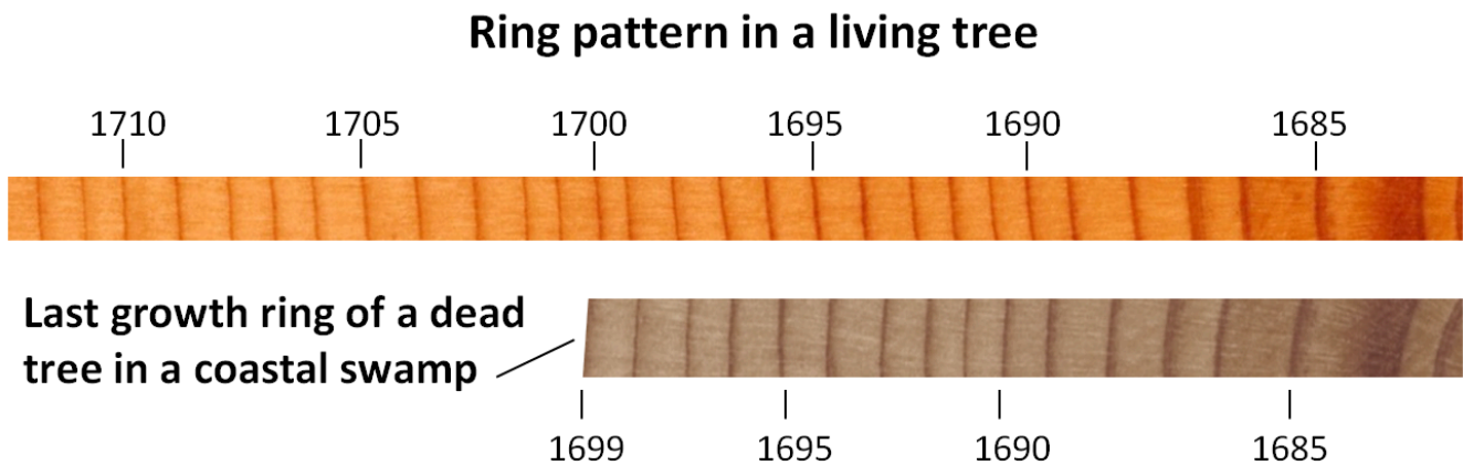
Figure 8.25.1 Example of tree-ring dating of dead trees.
