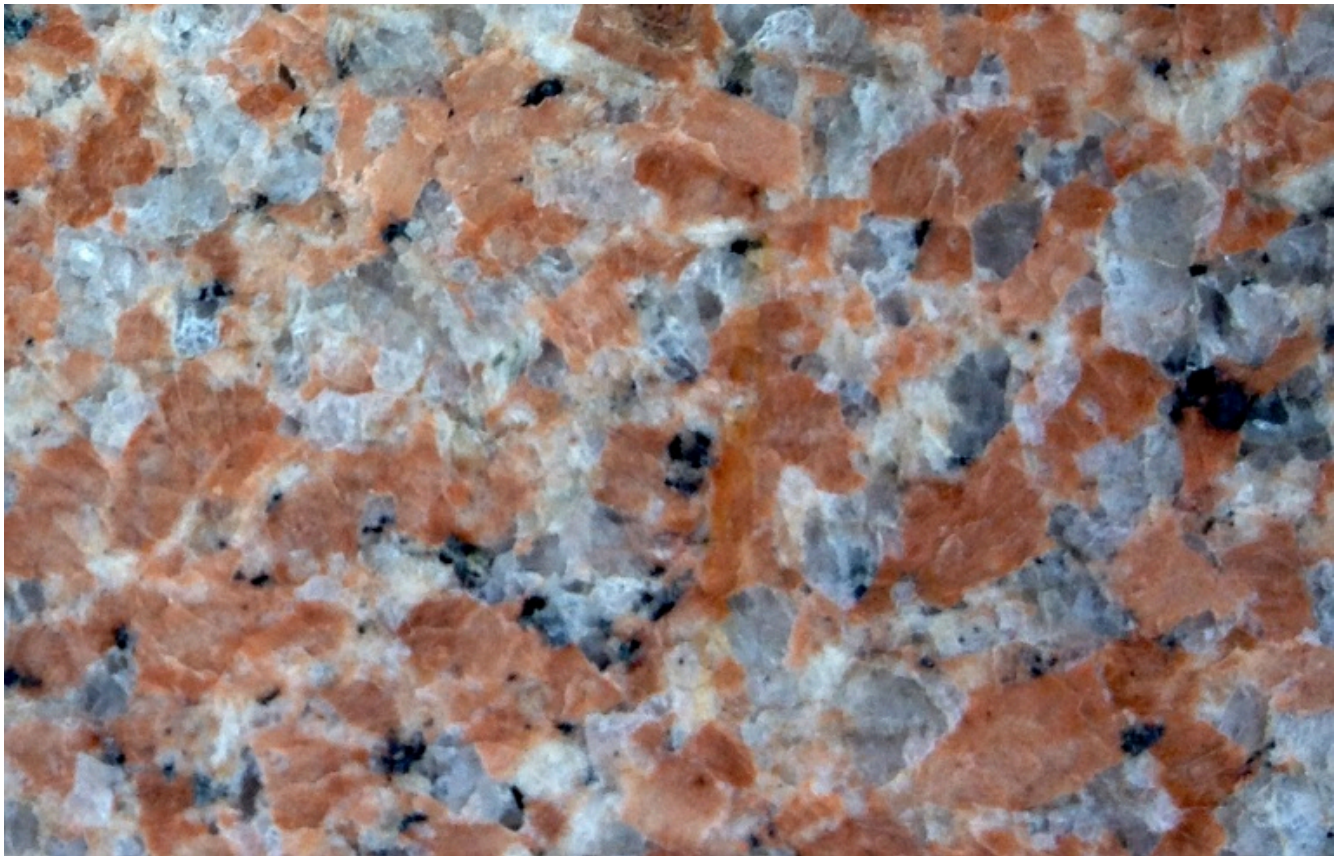
Figure 8.4.2 Crystals of potassium feldspar (pink) in a granitic rock are candidates for isotopic dating using the K-Ar method because they contained potassium and no argon when they formed.
