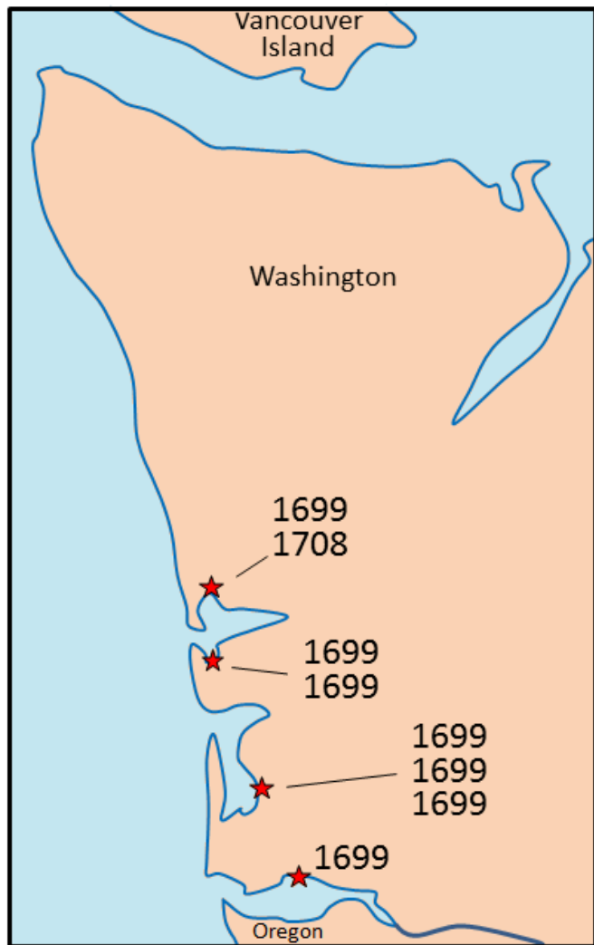
Figure 8.5.2 Sites in Washington where dead trees are present in coastal flats. The outermost wood of eight trees was dated using dendrochronology, and of these, seven died during the year 1699, suggesting that the land near to the coast was inundated by water at that time.
