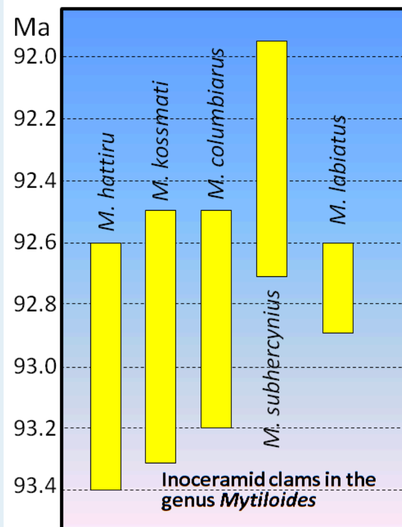
Figure 8.3.5 shows the age ranges for some late Cretaceous inoceramid clams in the genus Mytiloides :
