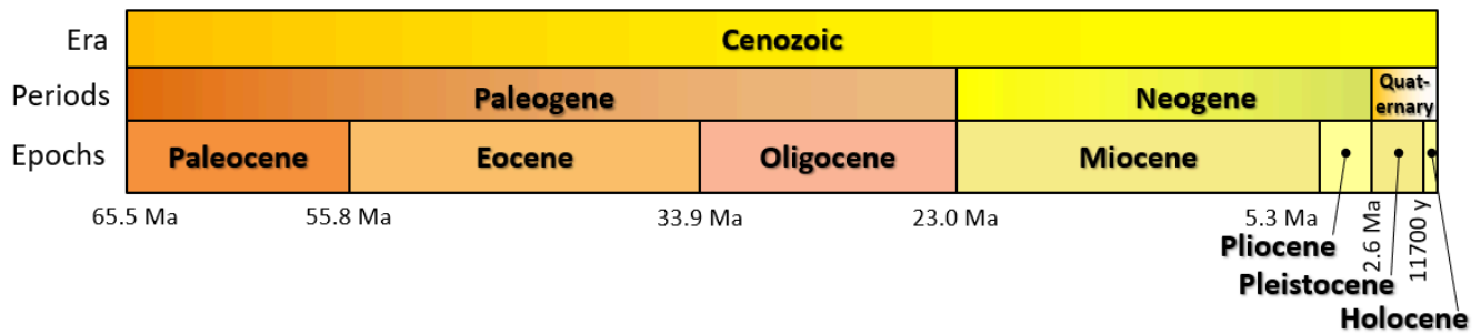
Figure 8.1.4 The periods (middle row) and epochs (bottom row) of the Cenozoic era. [Image Description]
