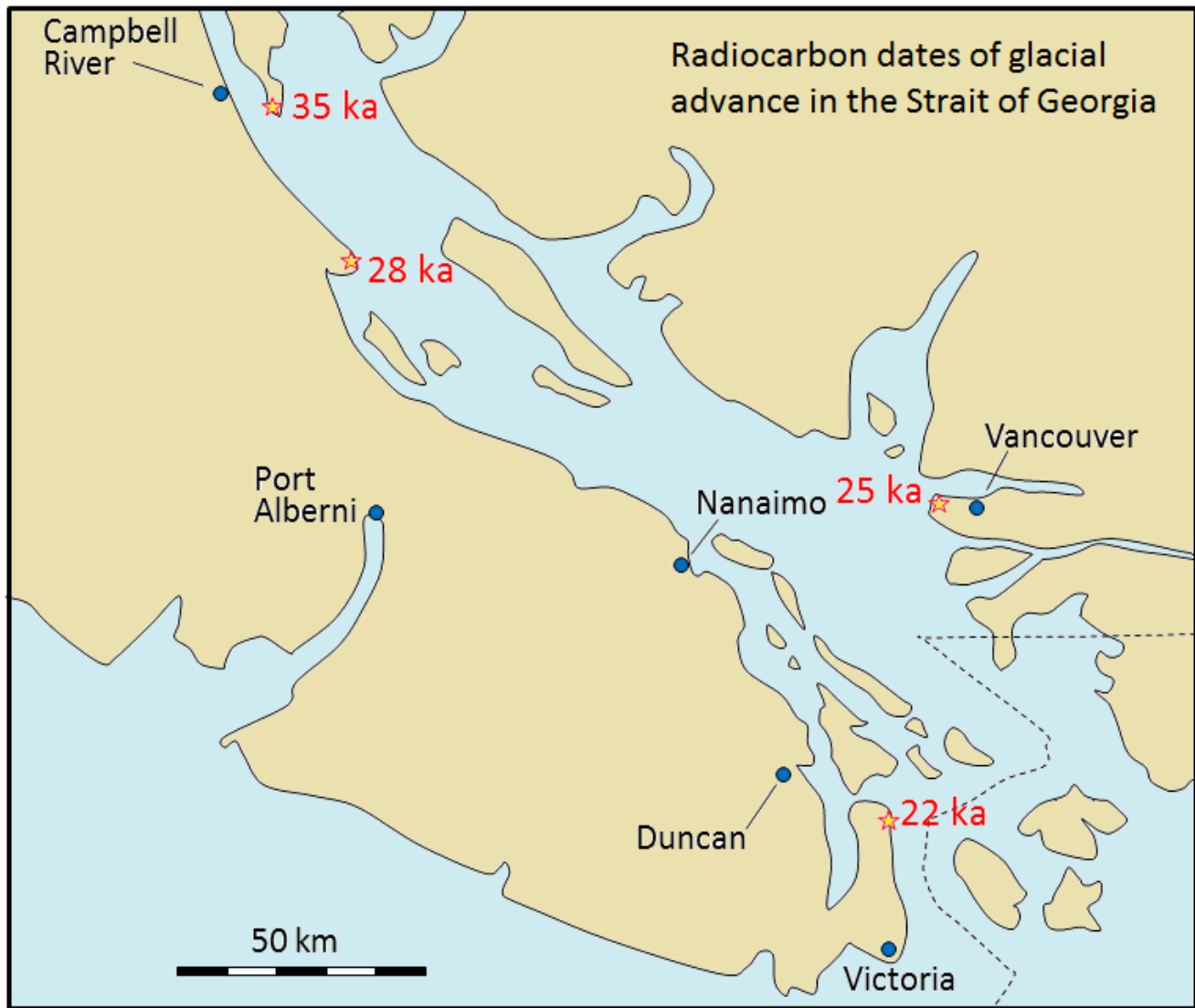
Figure 8.4.5 Radiocarbon dates on wood fragments in glacial sediments in the Strait of Georgia.
