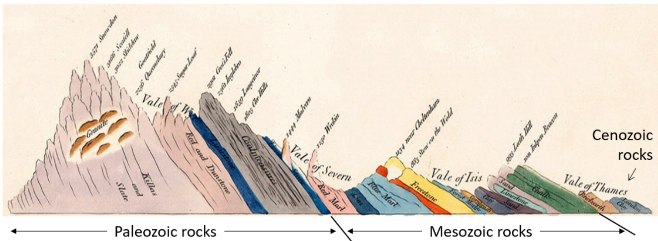
Figure 8.1.1 William Smith's "Sketch of the succession of strata and their relative altitudes," an inset on his geological map of England and Wales (with era names added).
