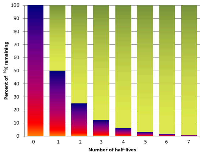
Figure 8.4.1 The decay of ^{40}\text{K} over time. Each half-life is 1.3 billion years, so after 3.9 billion years (three half-lives) 12.5% of the original ^{40}\text{K} will remain. The red-blue bars represent ^{40}\text{K} and the green-yellow bars represent ^{40}\text{Ar} . [Image Description]
