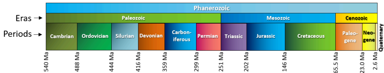
Figure 8.1.3 The eras (middle row) and periods (bottom row) of the Phanerozoic eon. [Image Description]
