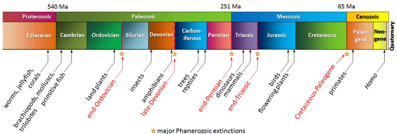
Figure 8.3.1 A summary of life on Earth during the late Proterozoic and the Phanerozoic. The top row shows geological eras, and the lower row shows the periods. [Image Description]
