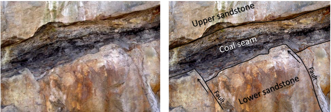
Figure 8.2.2 Superposition and cross-cutting relationships in Cretaceous Nanaimo Group rocks in Nanaimo, B.C. The coal seam is about 50 centimetres thick. The sequence of events is as follows: a) deposition of lower sandstone, b) faulting of lower sandstone, c) deposition of coal seam and d) deposition of upper sandstone.
