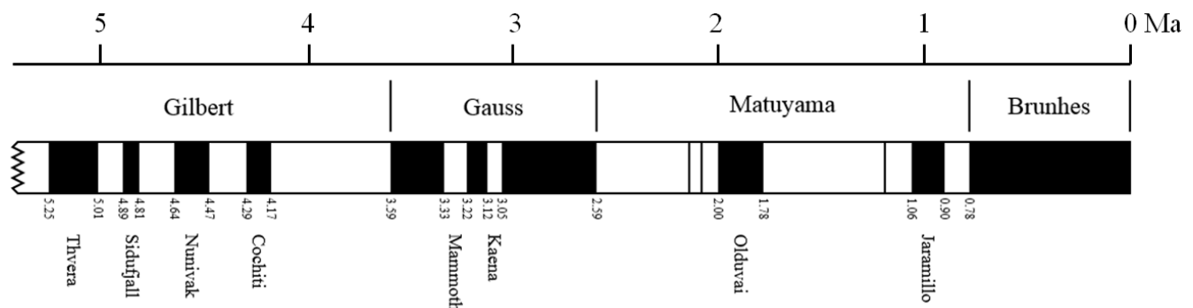
Figure 8.5.3 The last 5 Ma of magnetic field reversals.
