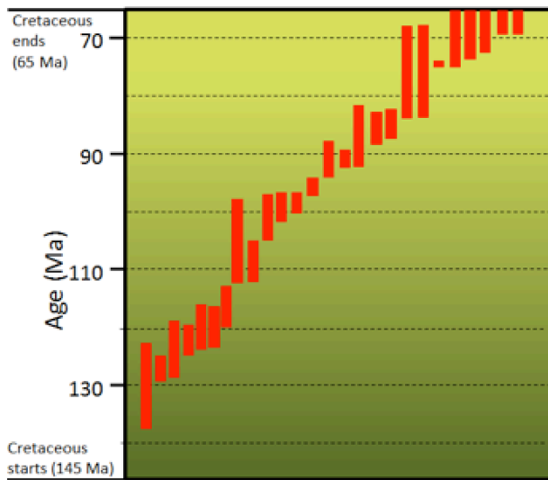
Time ranges of selected Cretaceous foraminifera species
