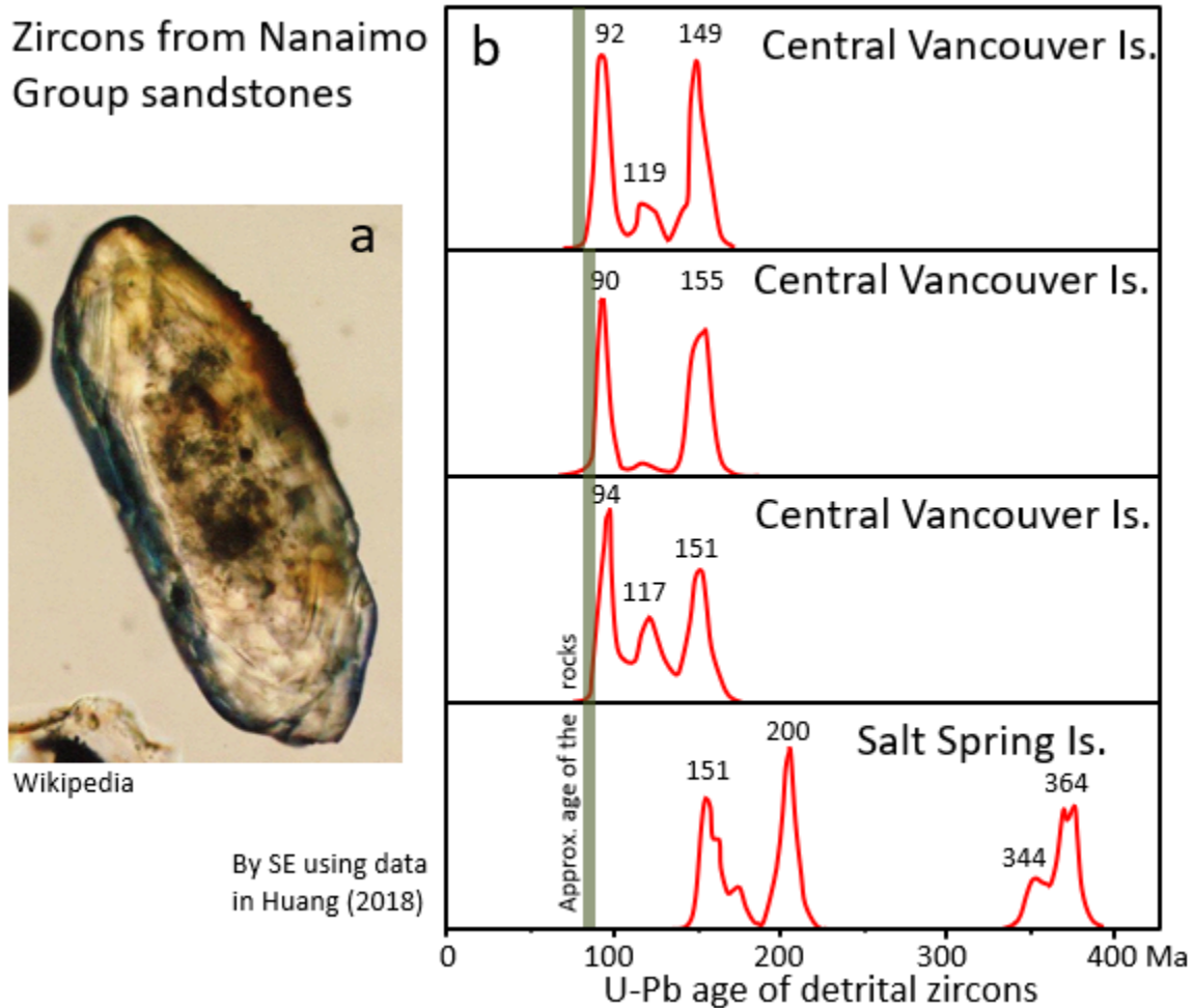
Figure 8.4.6 U-Pb dates for zircon samples from the Nanaimo Gp. (after Krause, 2018) a: a typical zircon clast (this one is about 1/4 mm long). b: plots of zircon ages for 4 sandstone samples.
