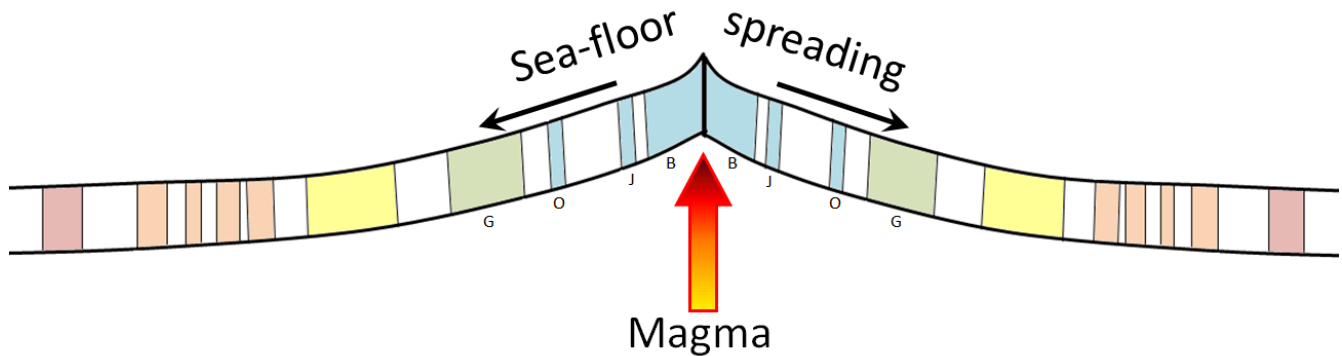
Figure 8.5.4 Depiction of the formation of magnetized oceanic crust at a spreading ridge. Coloured bars represent periods of normal magnetism, and the small capital letters denote the Brunhes, Jaramillo, Olduvai, and Gauss normal magnetic periods (see Figure 8.5.2).
