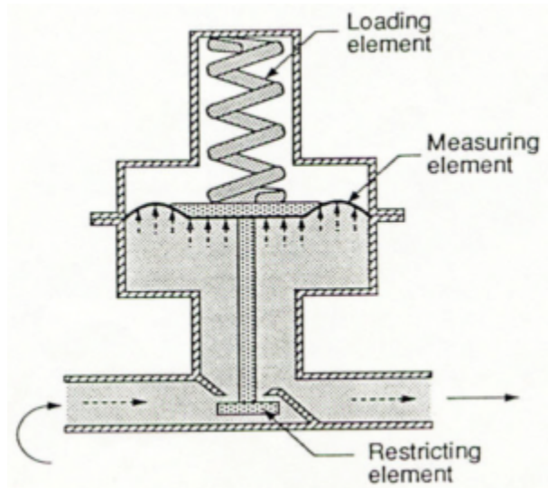
Figure 21. Operating elements
