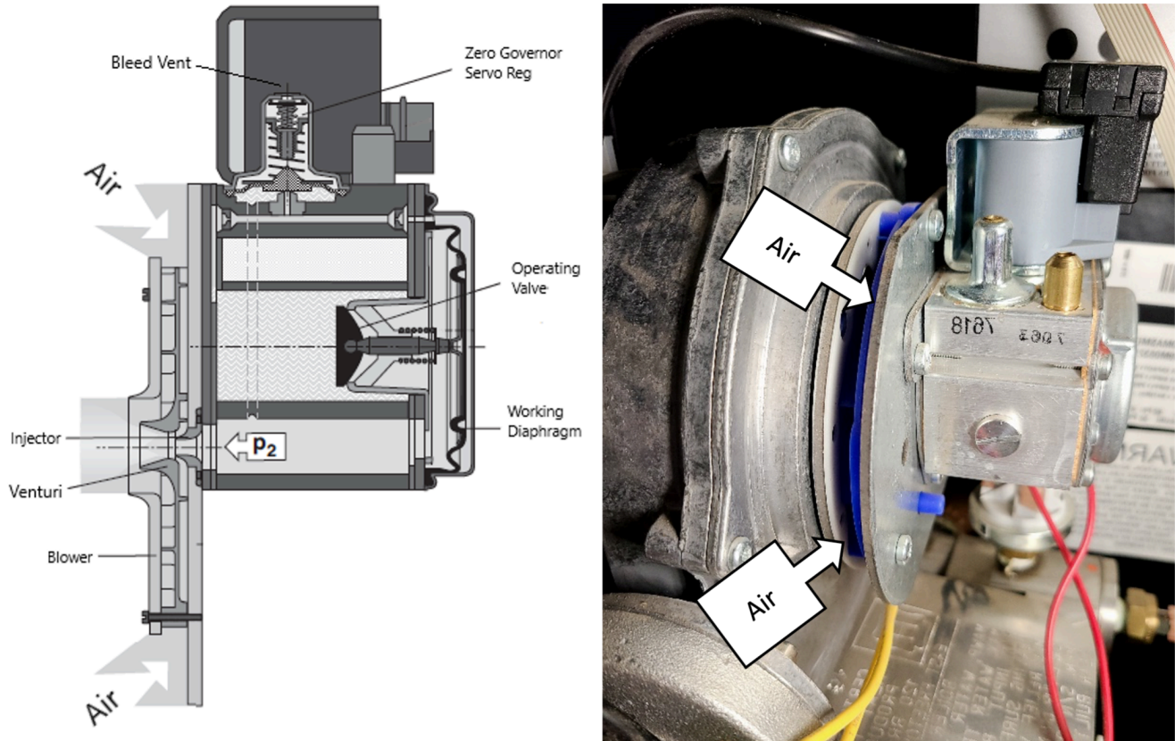
Figure 61. Modulating venturi burner
