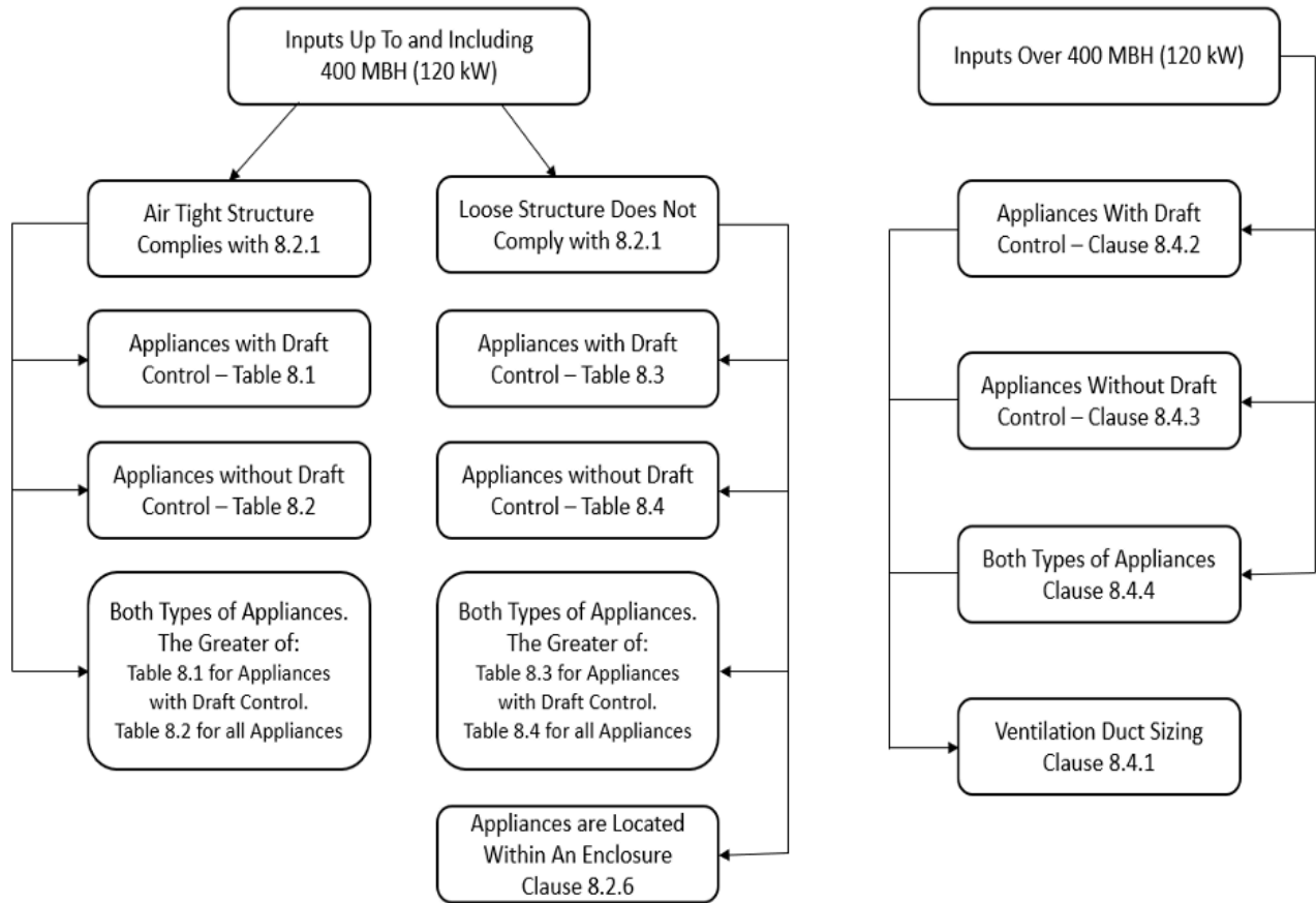
Figure 8. Air supply flow chart [Image Description]
