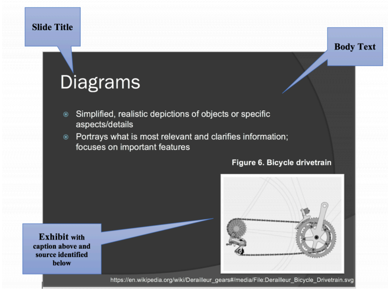
Figure 8.2.2 PowerPoint slide.
