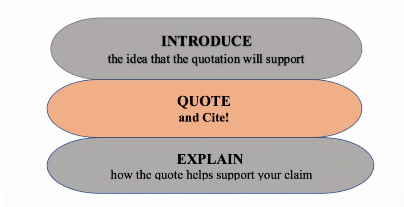
Figure C-1 Quotation sandwich.
