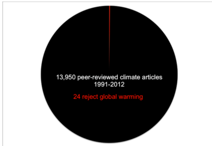
Figure 5.2.2 The number of articles that reject global warming out of all peer-reviewed climate articles within a 21 year time period.
